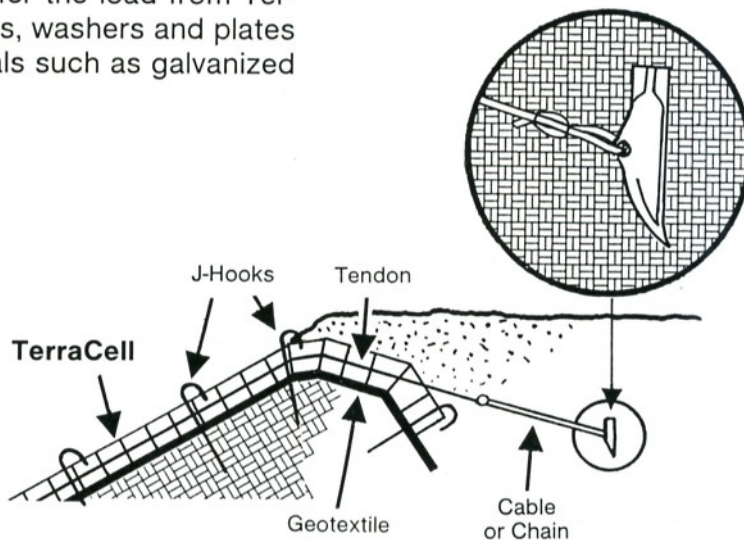
Supporting Structure: Harpoon-like System
